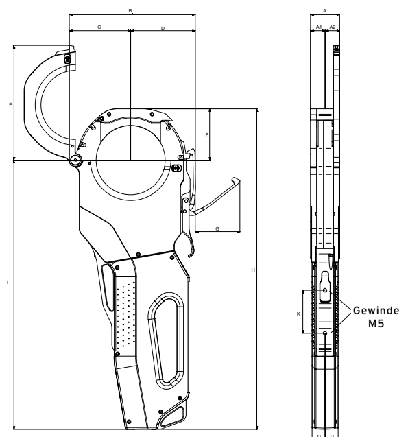
ORBIWELD X 3.0
