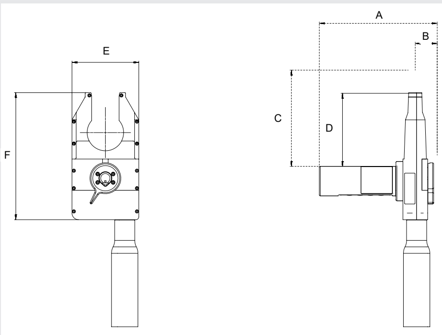
Dimensions OW 25 GC without cassette
